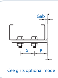
Cee girts standard mode
